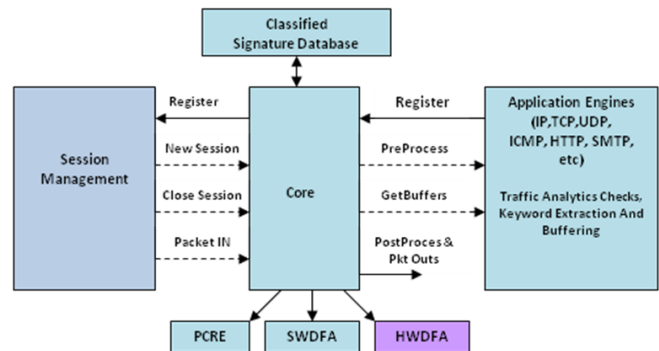
Block Diagram
